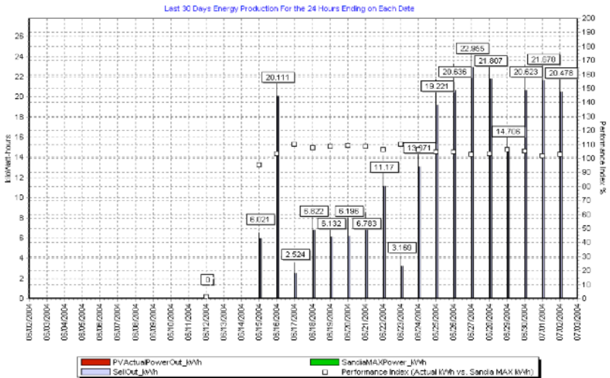
Above: Daily energy output for 3.8 kW PV 1 in June/July 2004. Note daily production varies considerably depending on weather, as seen mid-June (cloudy overcast) compared to sunny early July. Average is near 14 kWh/day over June/July for PV 1. These data were gathered just after a 1 st monitoring system was turned on, starting at mid chart, mid-June 2004.
